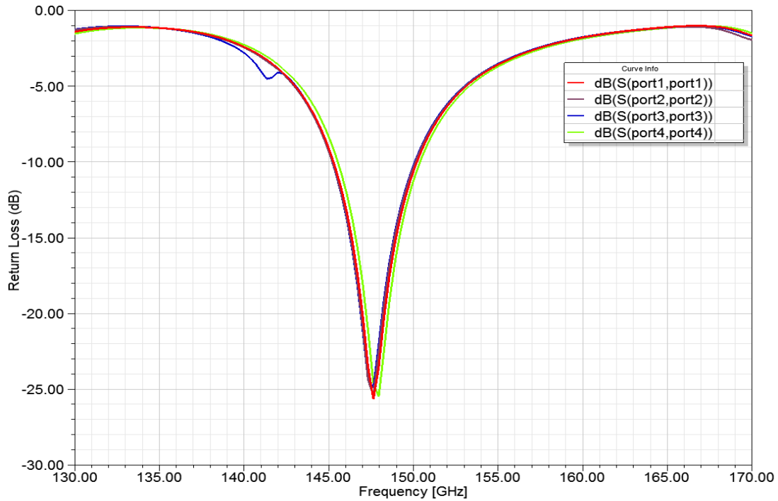
Figure 5.20. Return loss for log-spiral design in \text{dB}(S(Porti,Porti)) is 20\log_{10}(S_{ii}) , i=1, 2, 3, 4 .
