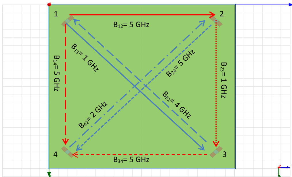
Figure 4.23. Channel assignment for the printed dipole model.
